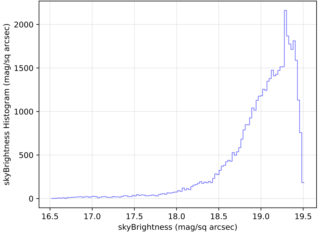
internal_u_expt27_nscale1.5v3.4_10yrs Yr 1 z band: skyBrightness Histogram
