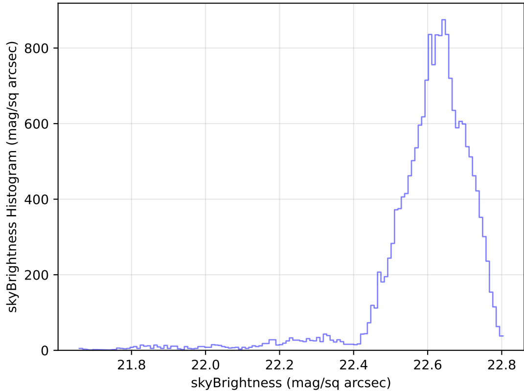
internal_u_expt27_nscale1.5v3.4_10yrs Yr 1 u band: skyBrightness Histogram
