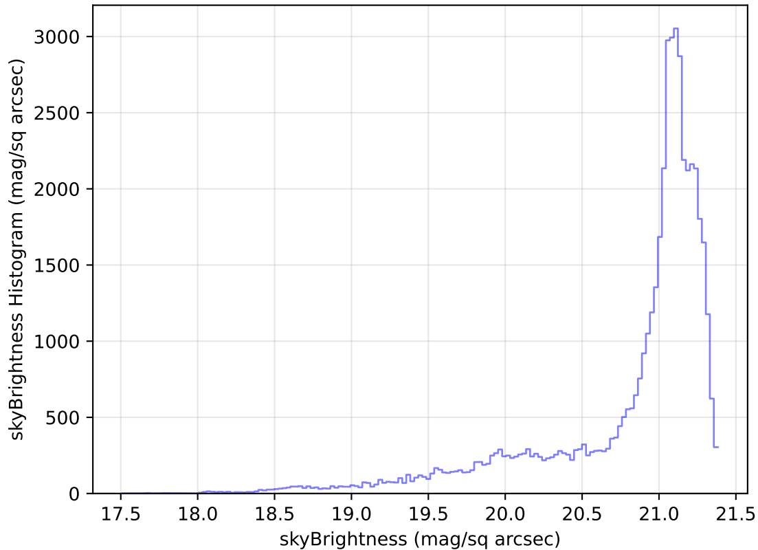
internal_u_expt27_nscale1.5v3.4_10yrs Yr 1 r band: skyBrightness Histogram
