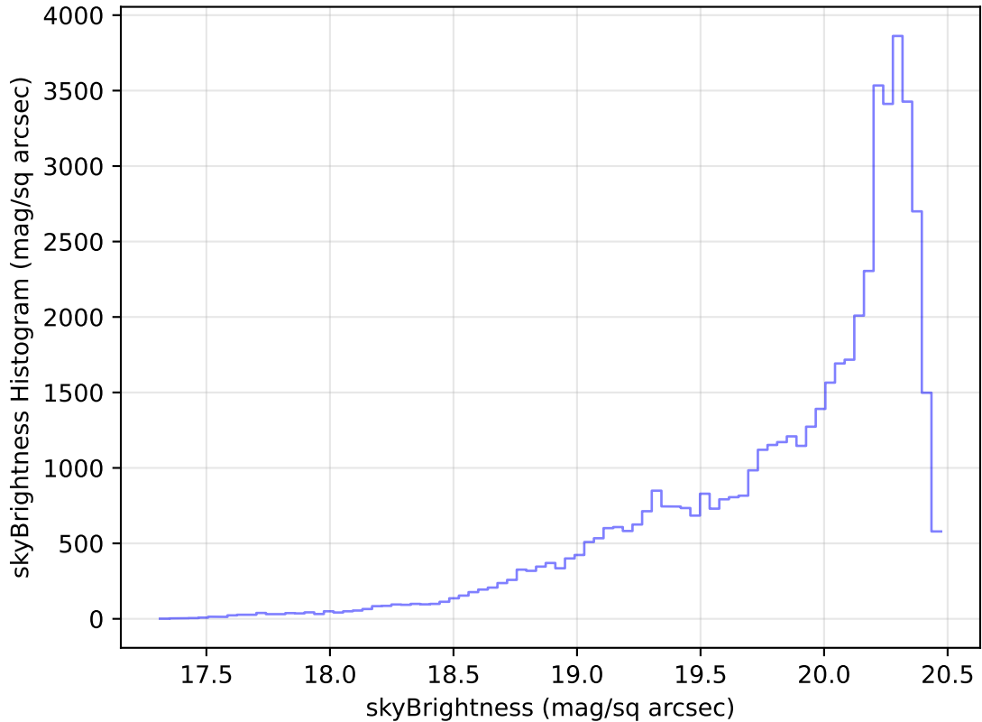
internal_u_expt27_nscale1.5v3.4_10yrs Yr 1 i band: skyBrightness Histogram
