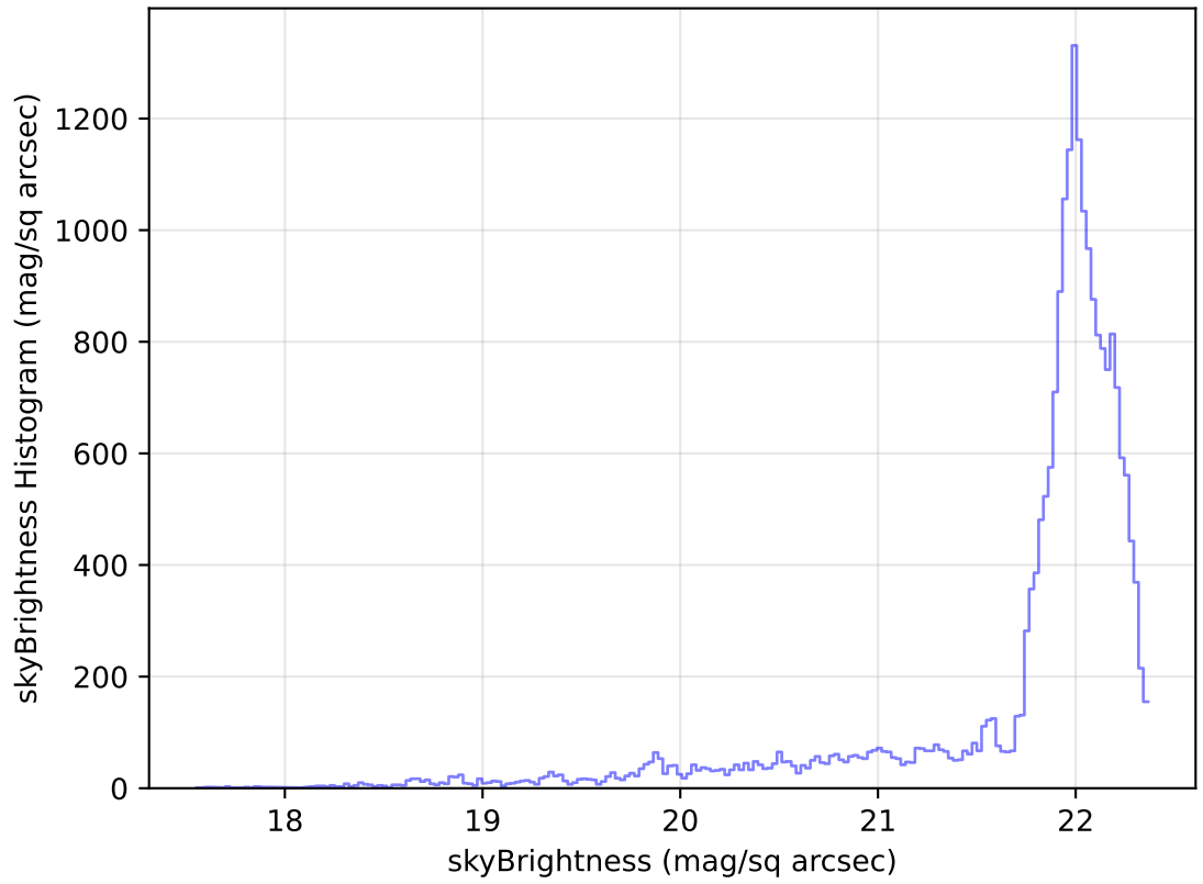
internal_u_expt27_nscale1.5v3.4_10yrs Yr 1 g band: skyBrightness Histogram
