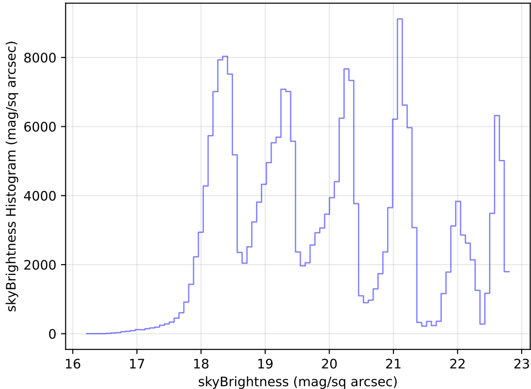
internal_u_expt27_nscale1.5v3.4_10yrs Yr 1 all bands: skyBrightness Histogram
