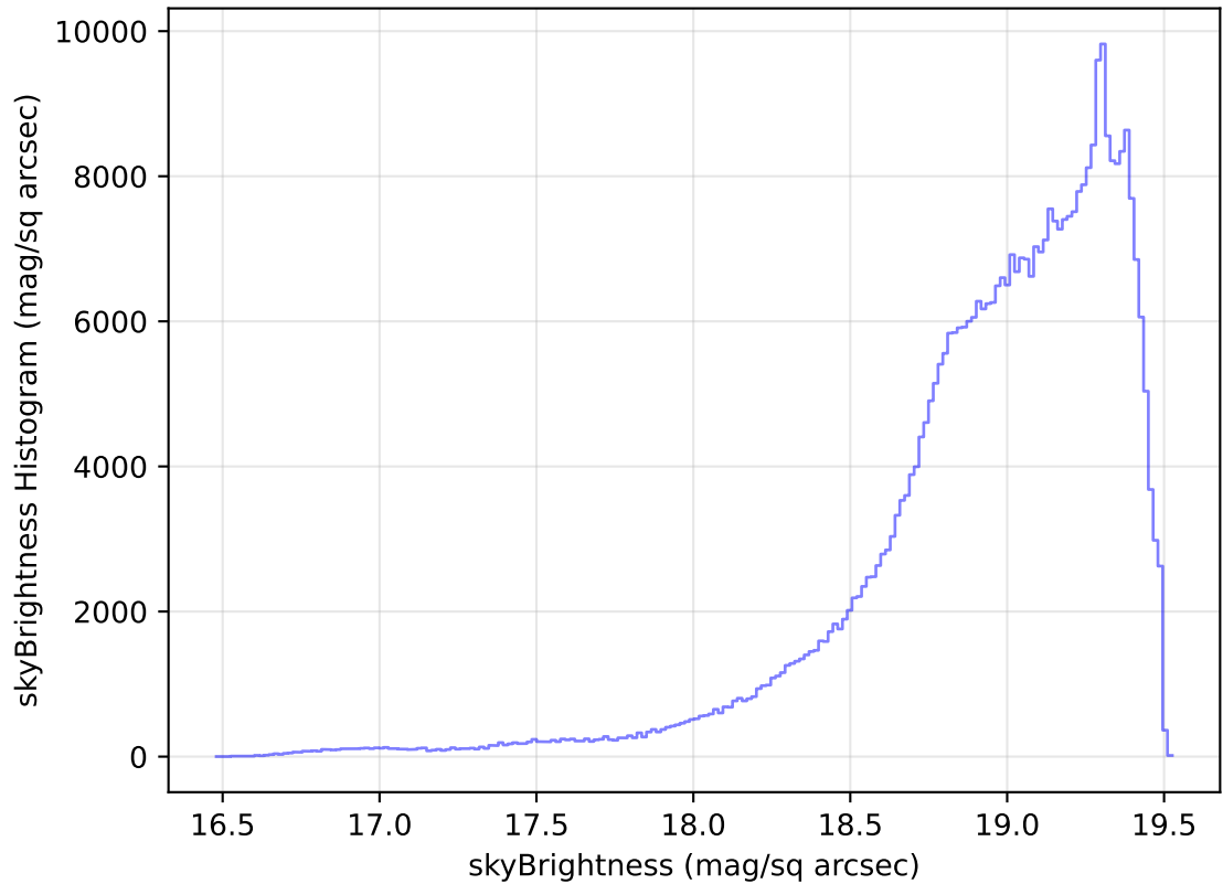
internal_u_expt27_nscale1.5v3.4_10yrs WFD z band: skyBrightness Histogram
