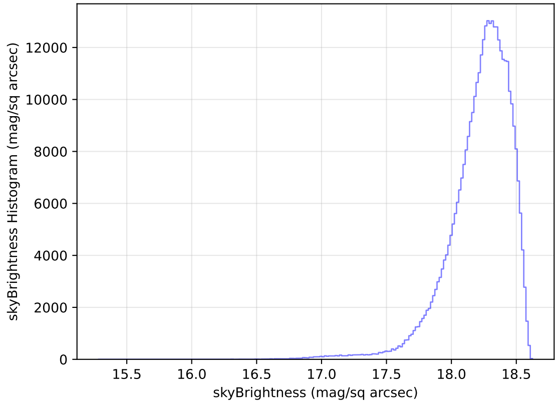
internal_u_expt27_nscale1.5v3.4_10yrs WFD y band: skyBrightness Histogram
