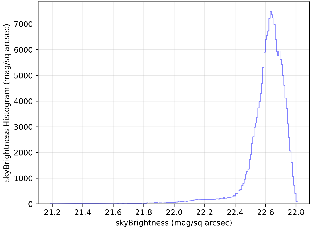
internal_u_expt27_nscale1.5v3.4_10yrs WFD u band: skyBrightness Histogram
