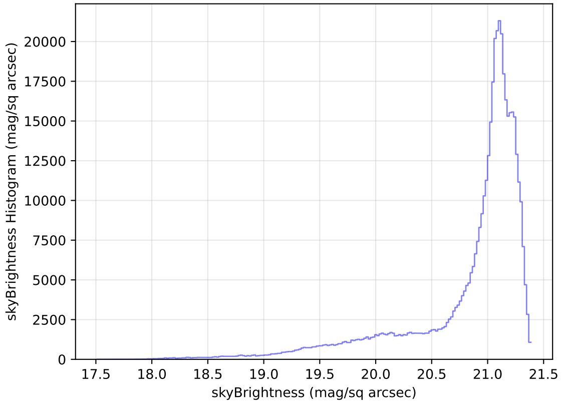
internal_u_expt27_nscale1.5v3.4_10yrs WFD r band: skyBrightness Histogram
