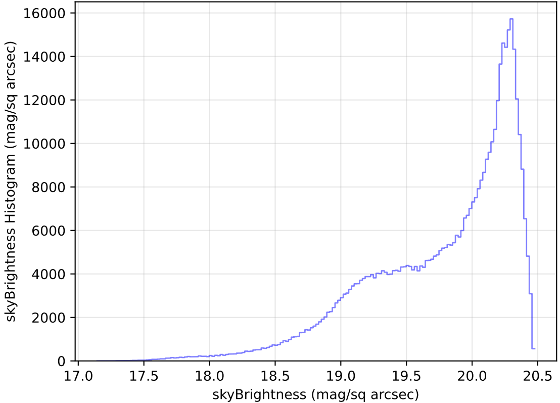
internal_u_expt27_nscale1.5v3.4_10yrs WFD i band: skyBrightness Histogram
