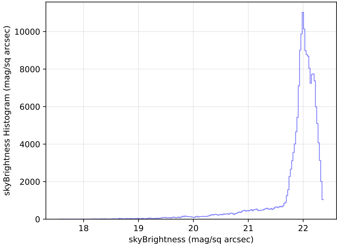
internal_u_expt27_nscale1.5v3.4_10yrs WFD g band: skyBrightness Histogram
