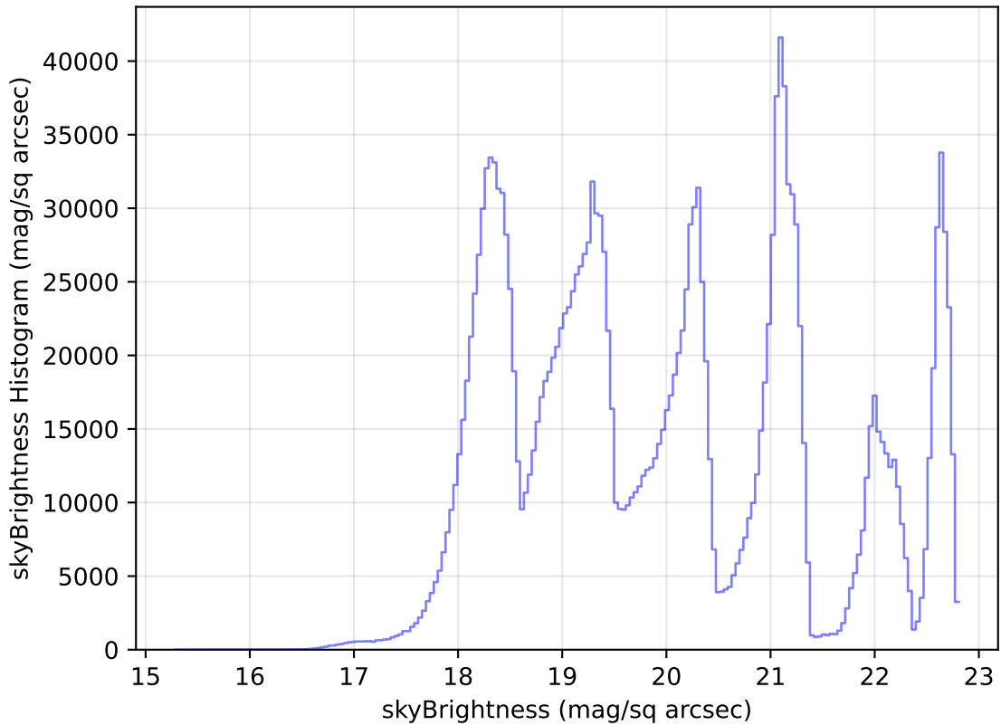
internal_u_expt27_nscale1.5v3.4_10yrs WFD all bands: skyBrightness Histogram
