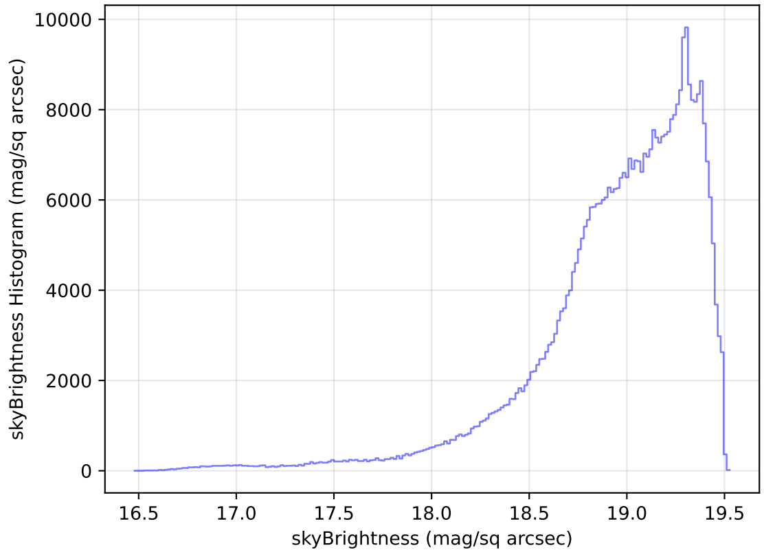
internal_u_expt27_nscale1.5v3.4_10yrs All sky z band: skyBrightness Histogram
