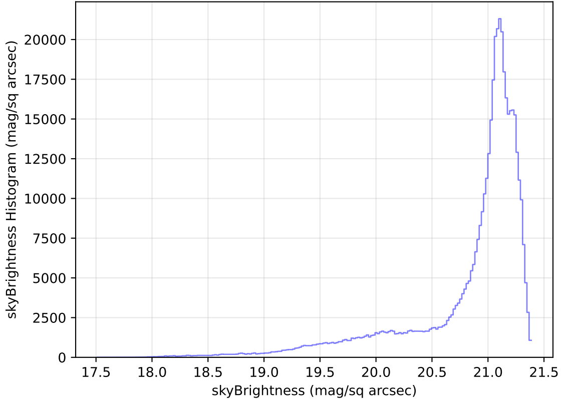
internal_u_expt27_nscale1.5v3.4_10yrs All sky r band: skyBrightness Histogram
