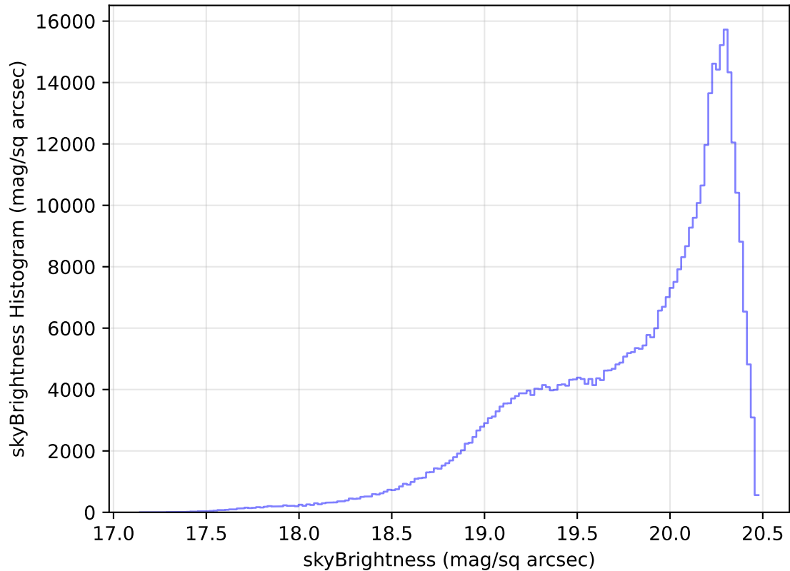
internal_u_expt27_nscale1.5v3.4_10yrs All sky i band: skyBrightness Histogram
