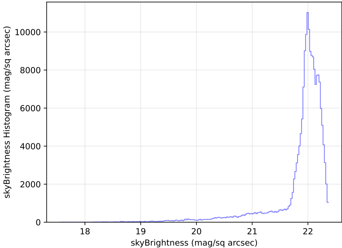
internal_u_expt27_nscale1.5v3.4_10yrs All sky g band: skyBrightness Histogram
