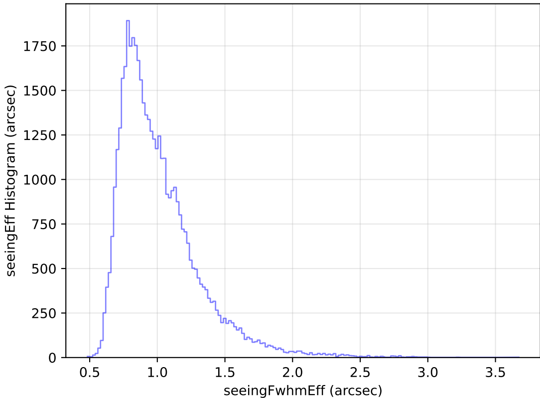
internal_u_expt27_nscale1.5v3.4_10yrs Yr 1 z band: seeingEff Histogram
