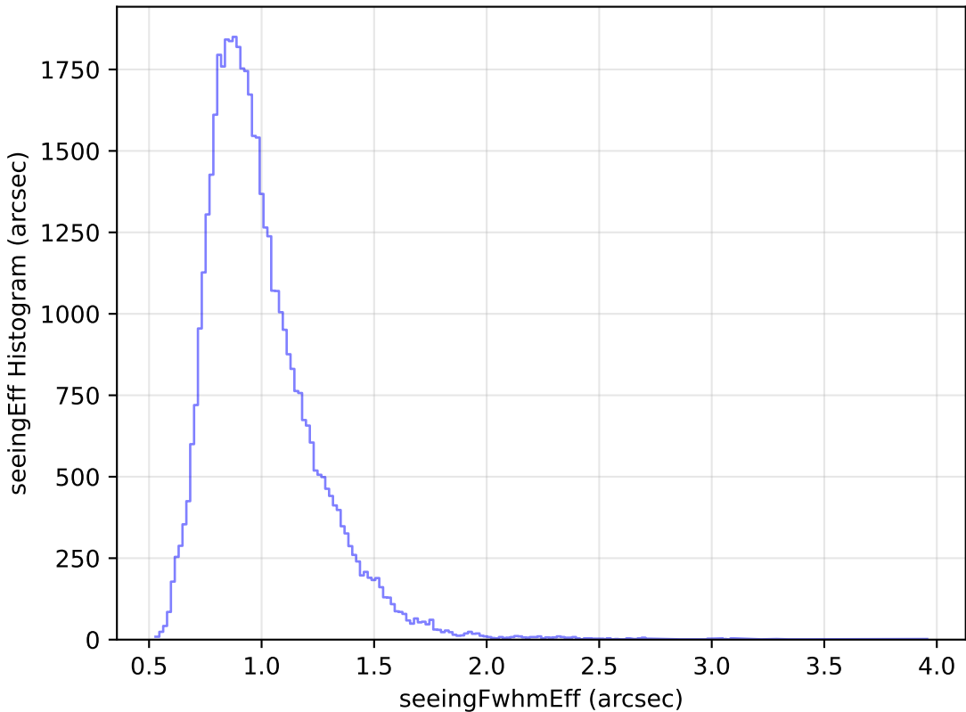
internal_u_expt27_nscale1.5v3.4_10yrs Yr 1 y band: seeingEff Histogram
