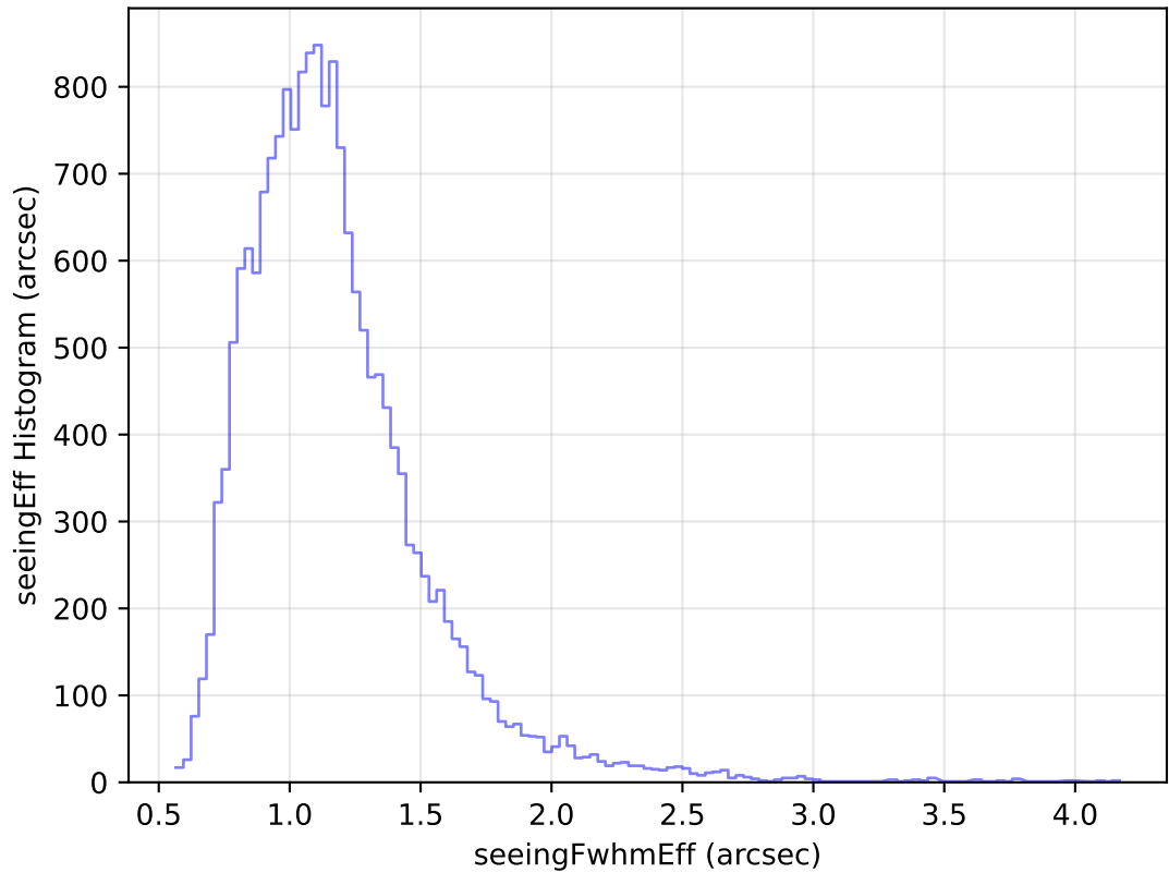
internal_u_expt27_nscale1.5v3.4_10yrs Yr 1 u band: seeingEff Histogram
