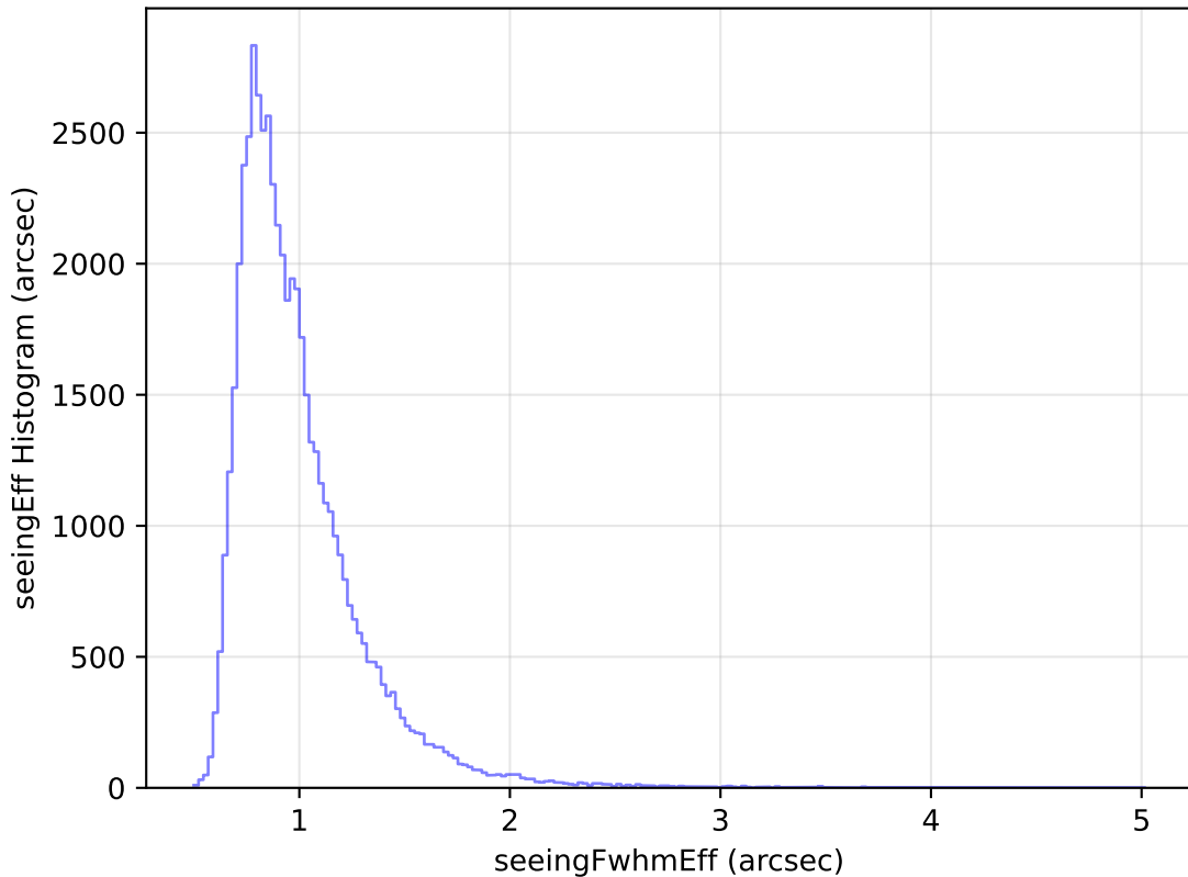
internal_u_expt27_nscale1.5v3.4_10yrs Yr 1 i band: seeingEff Histogram
