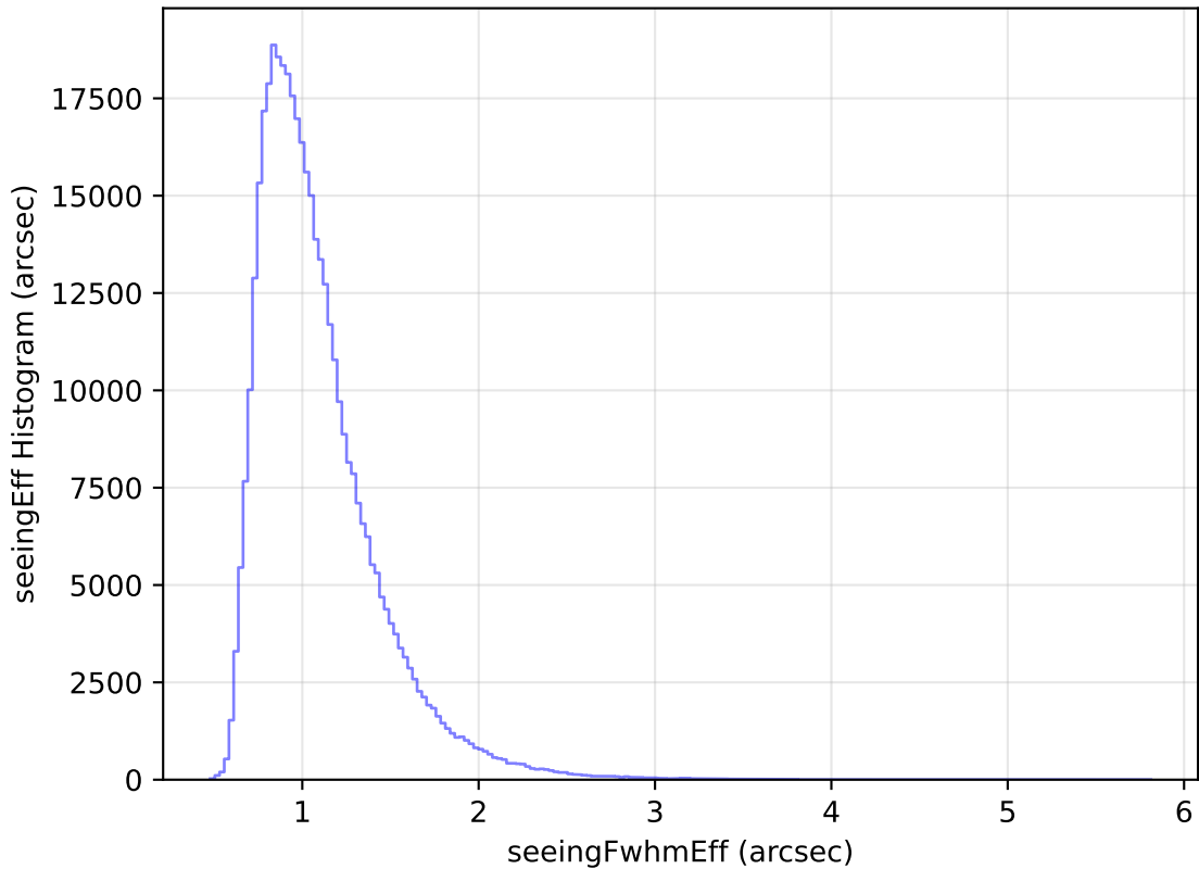
internal_u_expt27_nscale1.5v3.4_10yrs WFD z band: seeingEff Histogram
