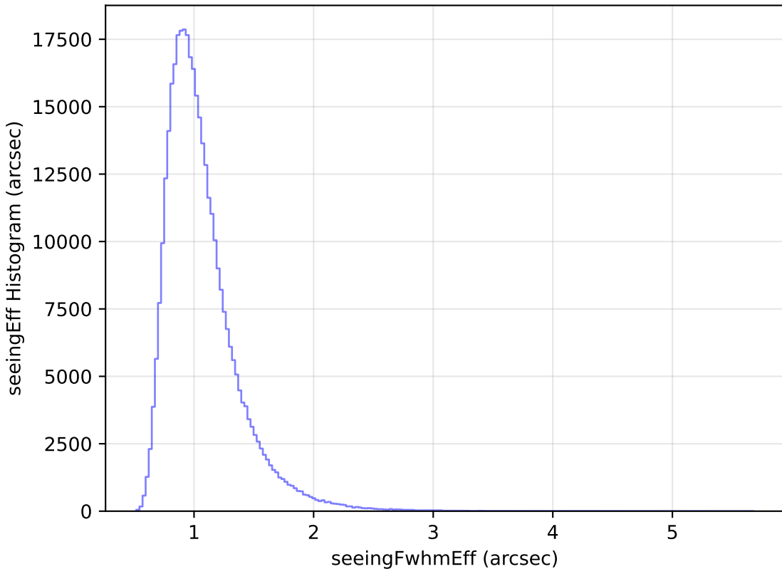
internal_u_expt27_nscale1.5v3.4_10yrs WFD y band: seeingEff Histogram
