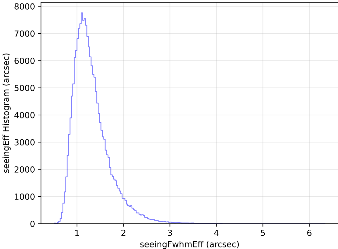
internal_u_expt27_nscale1.5v3.4_10yrs WFD u band: seeingEff Histogram
