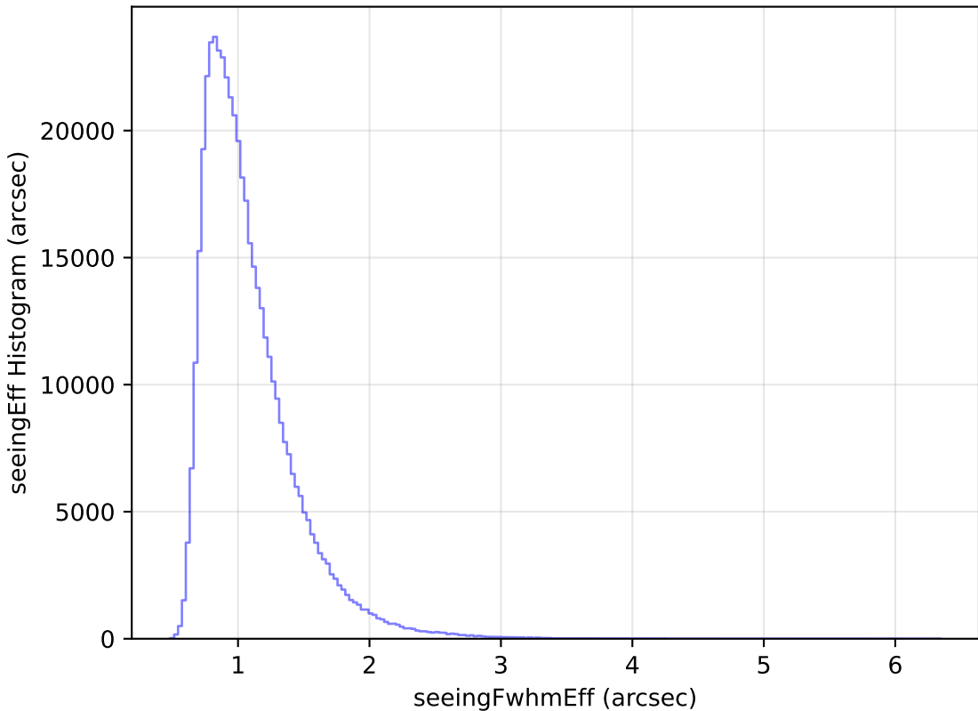
internal_u_expt27_nscale1.5v3.4_10yrs WFD i band: seeingEff Histogram
