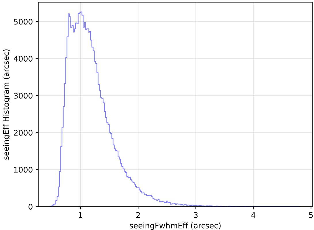
internal_u_expt27_nscale1.5v3.4_10yrs WFD g band: seeingEff Histogram
