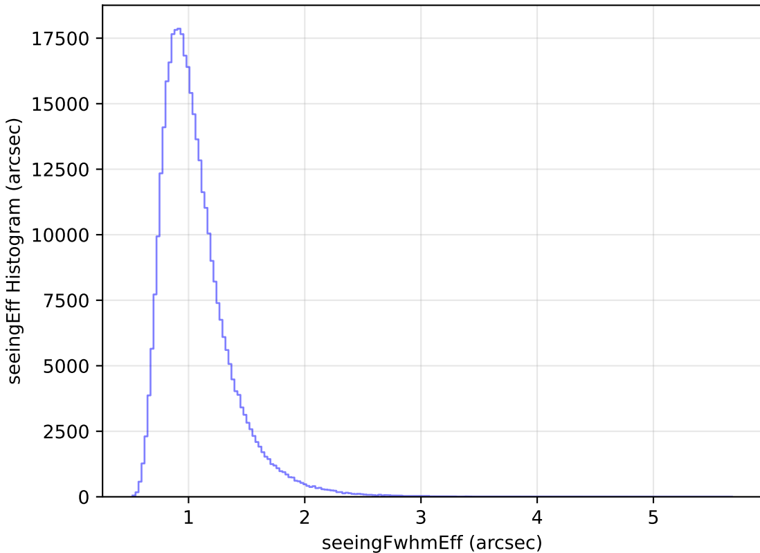
internal_u_expt27_nscale1.5v3.4_10yrs All sky y band: seeingEff Histogram
