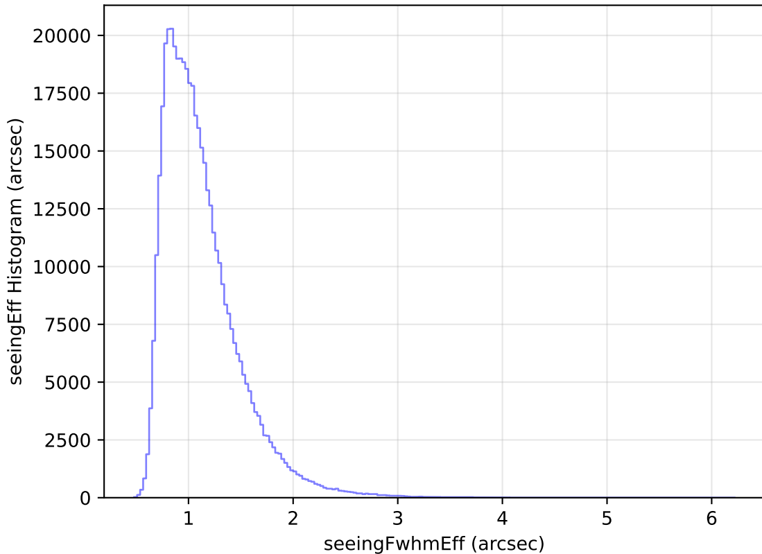
internal_u_expt27_nscale1.5v3.4_10yrs All sky r band: seeingEff Histogram
