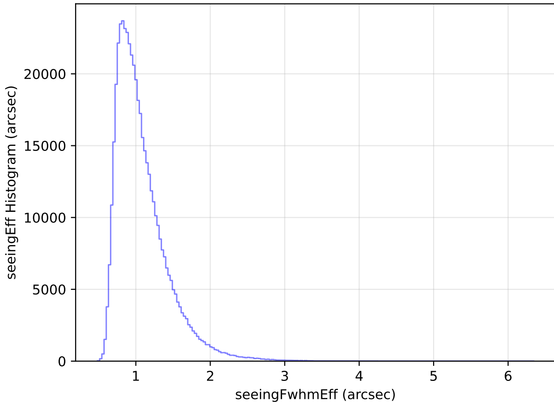
internal_u_expt27_nscale1.5v3.4_10yrs All sky i band: seeingEff Histogram
