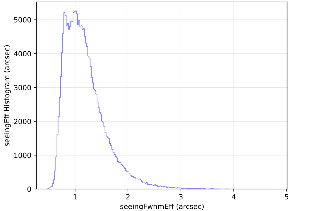
internal_u_expt27_nscale1.5v3.4_10yrs All sky g band: seeingEff Histogram
