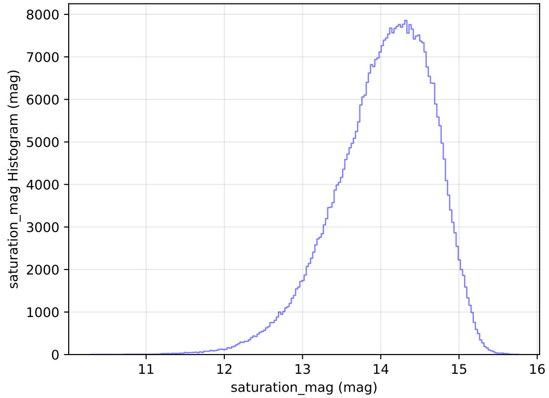
internal_u_expt27_nscale1.5v3.4_10yrs WFD z band: saturation_mag Histogram
