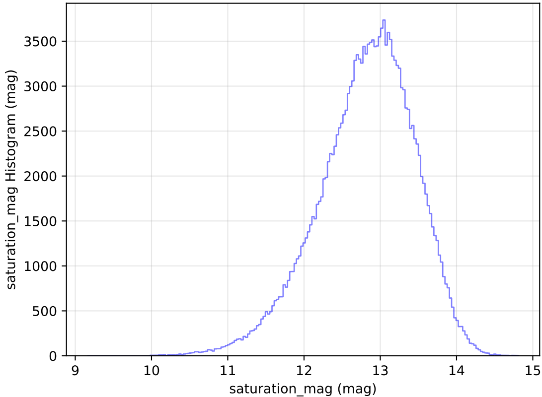
internal_u_expt27_nscale1.5v3.4_10yrs WFD u band: saturation_mag Histogram
