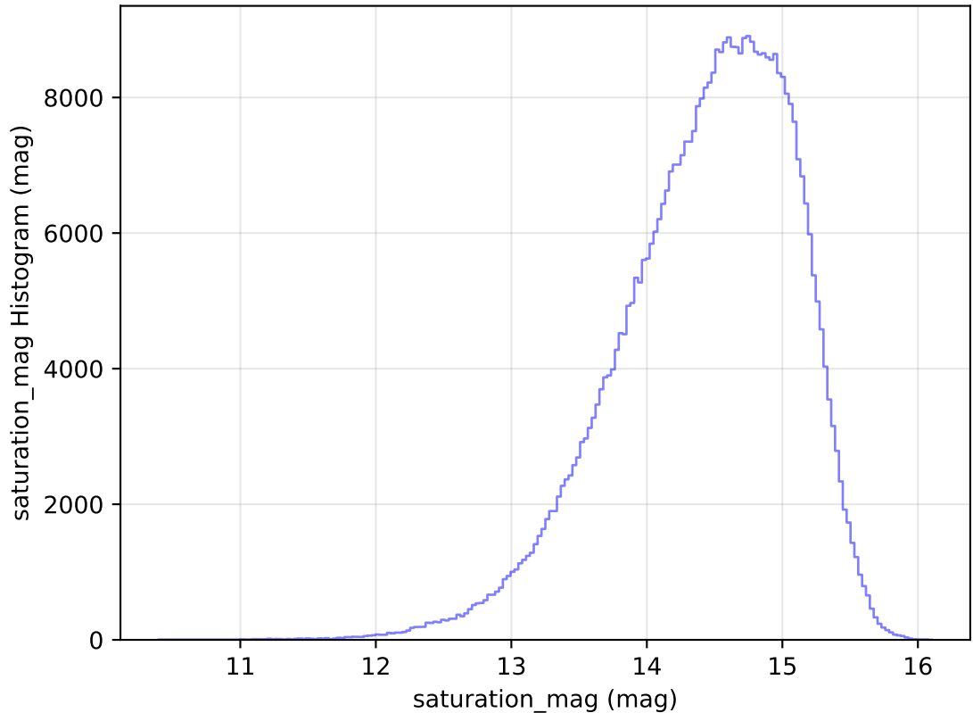
internal_u_expt27_nscale1.5v3.4_10yrs WFD i band: saturation_mag Histogram
