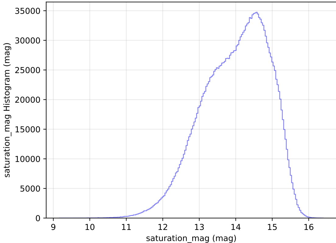
internal_u_expt27_nscale1.5v3.4_10yrs WFD all bands: saturation_mag Histogram
