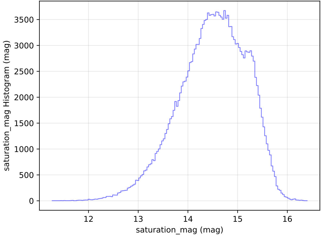
internal_u_expt27_nscale1.5v3.4_10yrs All sky g band: saturation_mag Histogram
