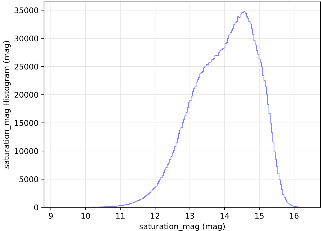
internal_u_expt27_nscale1.5v3.4_10yrs All sky all bands: saturation_mag Histogram
