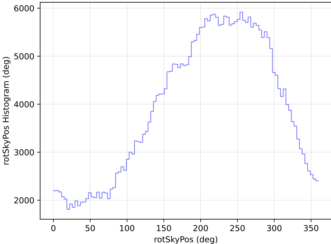
internal_u_expt27_nscale1.5v3.4_10yrs WFD y band: rotSkyPos Histogram
