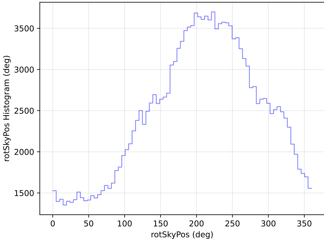
internal_u_expt27_nscale1.5v3.4_10yrs WFD u band: rotSkyPos Histogram
