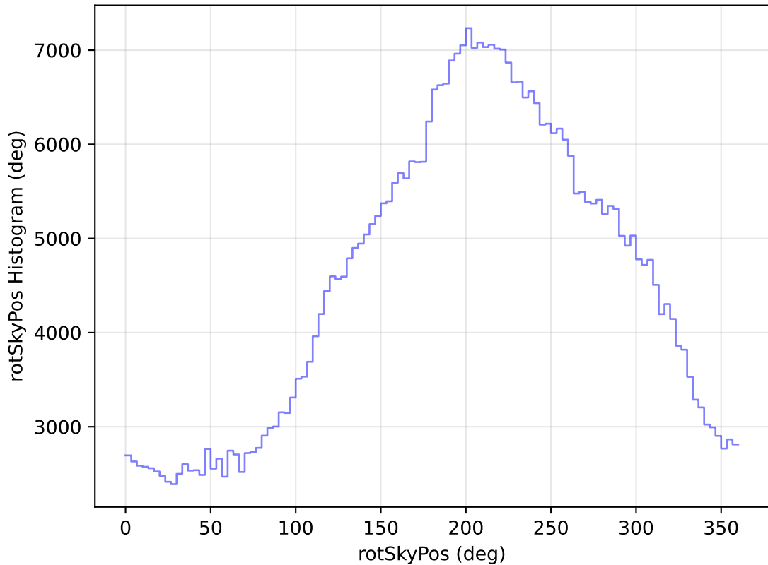
internal_u_expt27_nscale1.5v3.4_10yrs WFD i band: rotSkyPos Histogram
