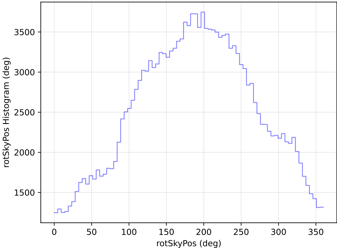
internal_u_expt27_nscale1.5v3.4_10yrs WFD g band: rotSkyPos Histogram
