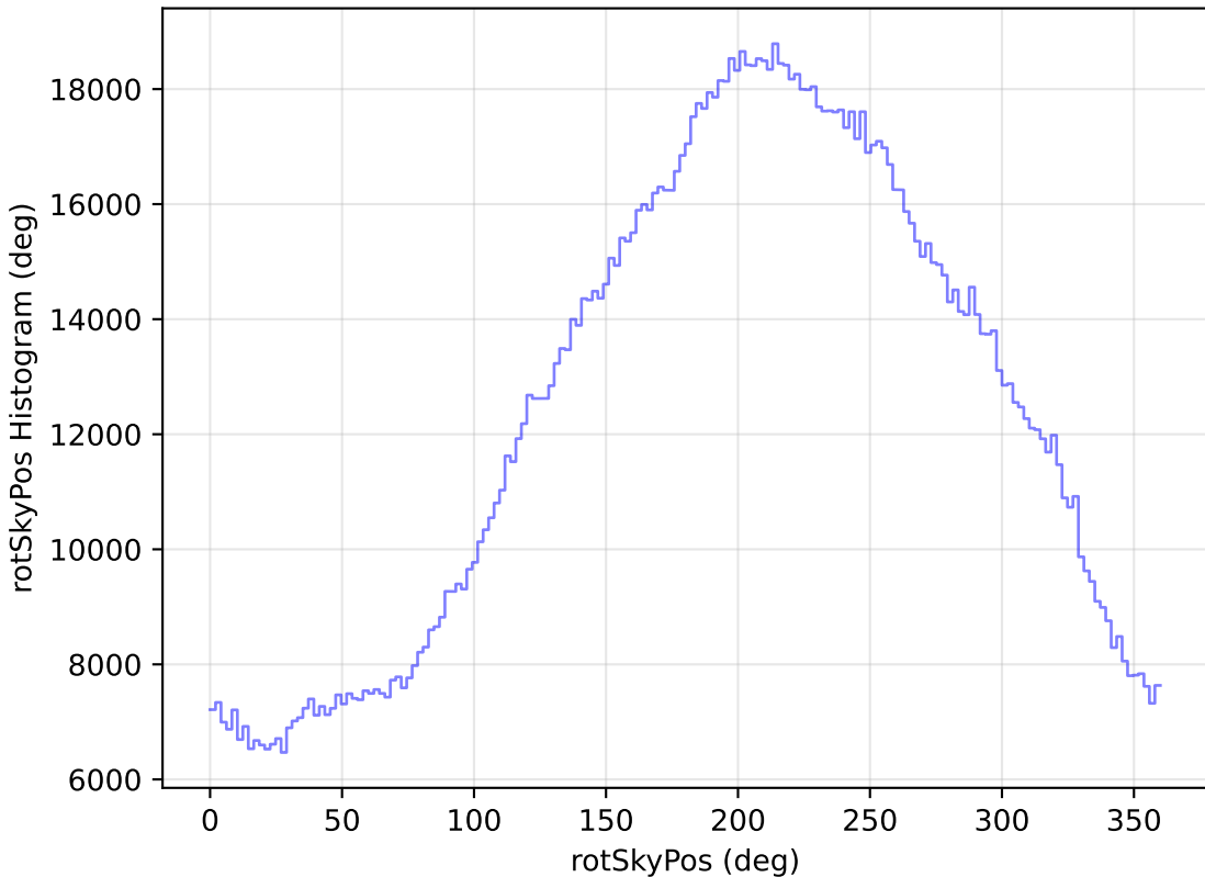
internal_u_expt27_nscale1.5v3.4_10yrs WFD all bands: rotSkyPos Histogram
