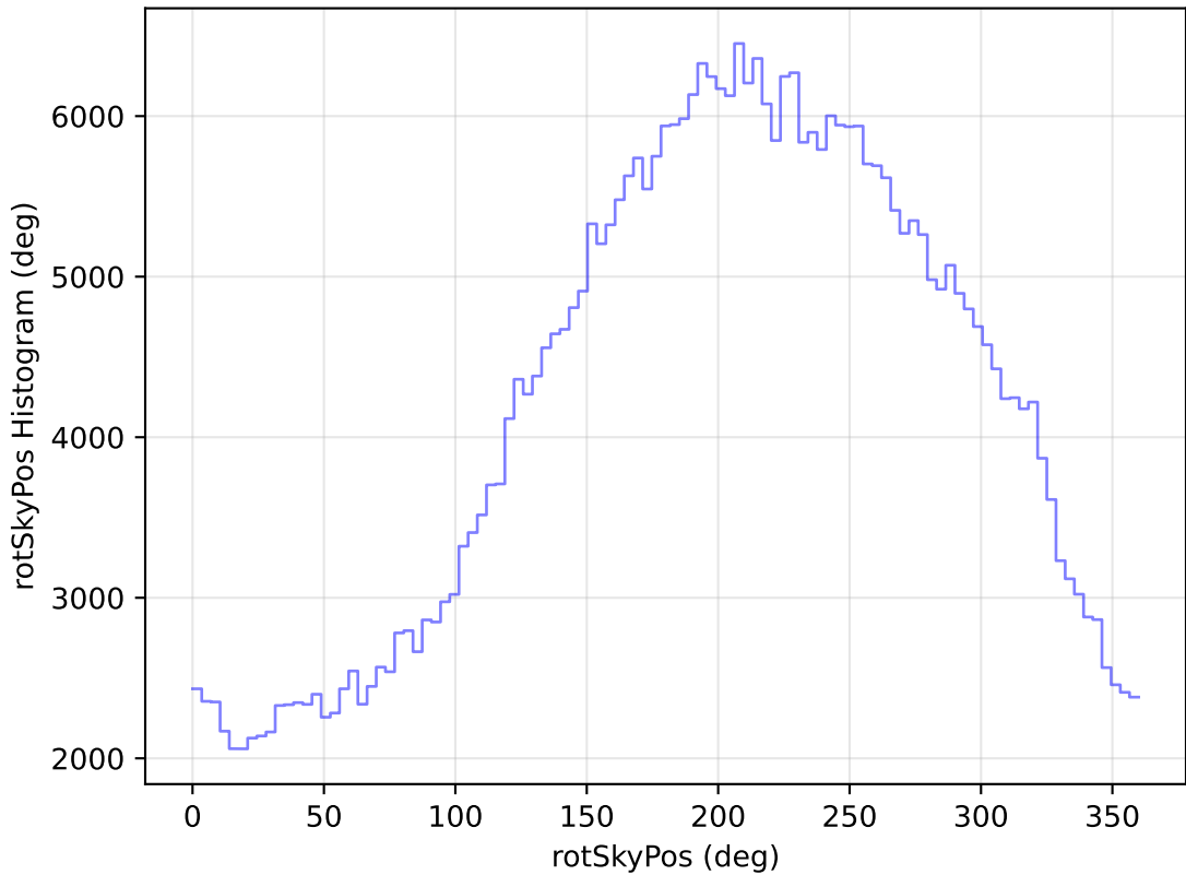
internal_u_expt27_nscale1.5v3.4_10yrs All sky z band: rotSkyPos Histogram
