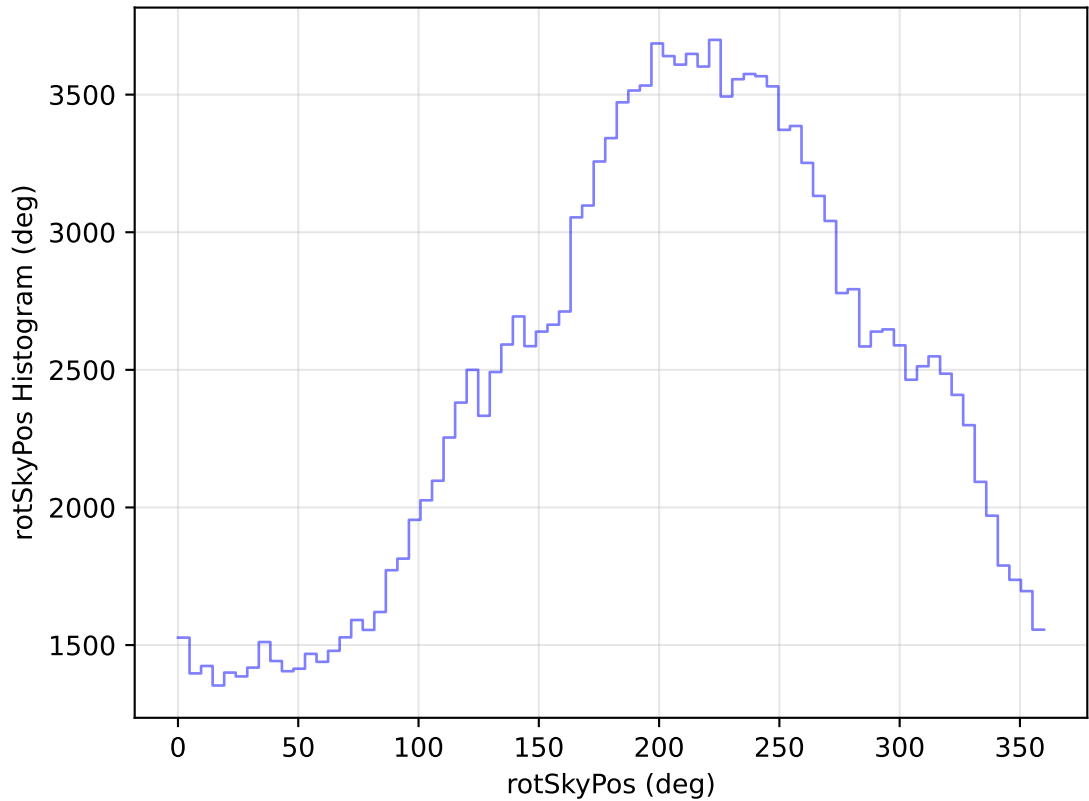
internal_u_expt27_nscale1.5v3.4_10yrs All sky u band: rotSkyPos Histogram
