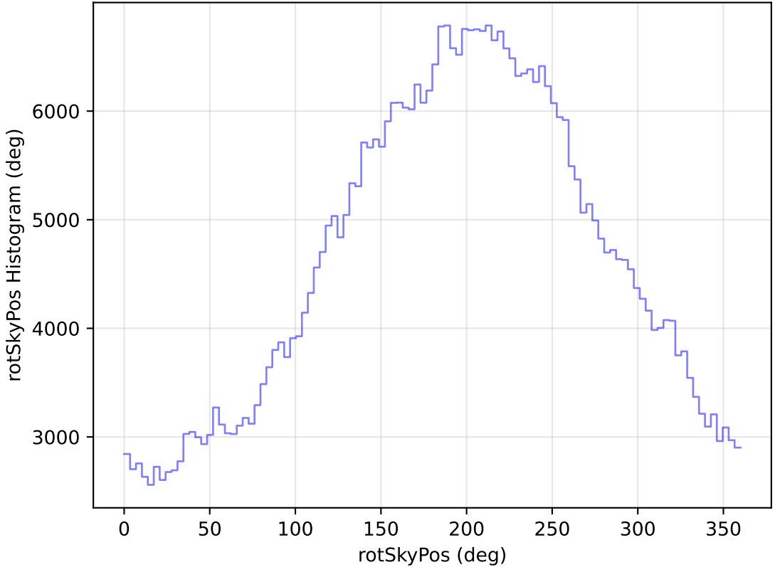
internal_u_expt27_nscale1.5v3.4_10yrs All sky r band: rotSkyPos Histogram
