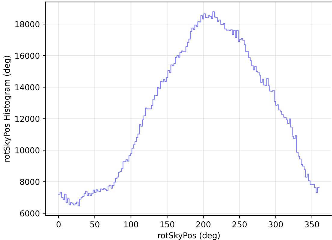
internal_u_expt27_nscale1.5v3.4_10yrs All sky all bands: rotSkyPos Histogram
