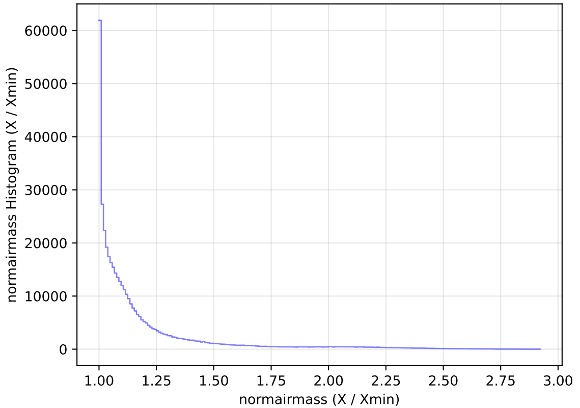
internal_u_expt27_nscale1.5v3.4_10yrs WFD z band: normairmass Histogram
