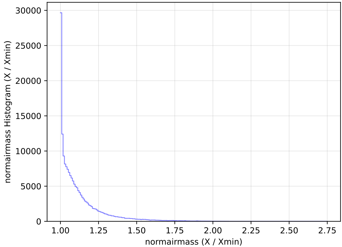
internal_u_expt27_nscale1.5v3.4_10yrs WFD u band: normairmass Histogram
