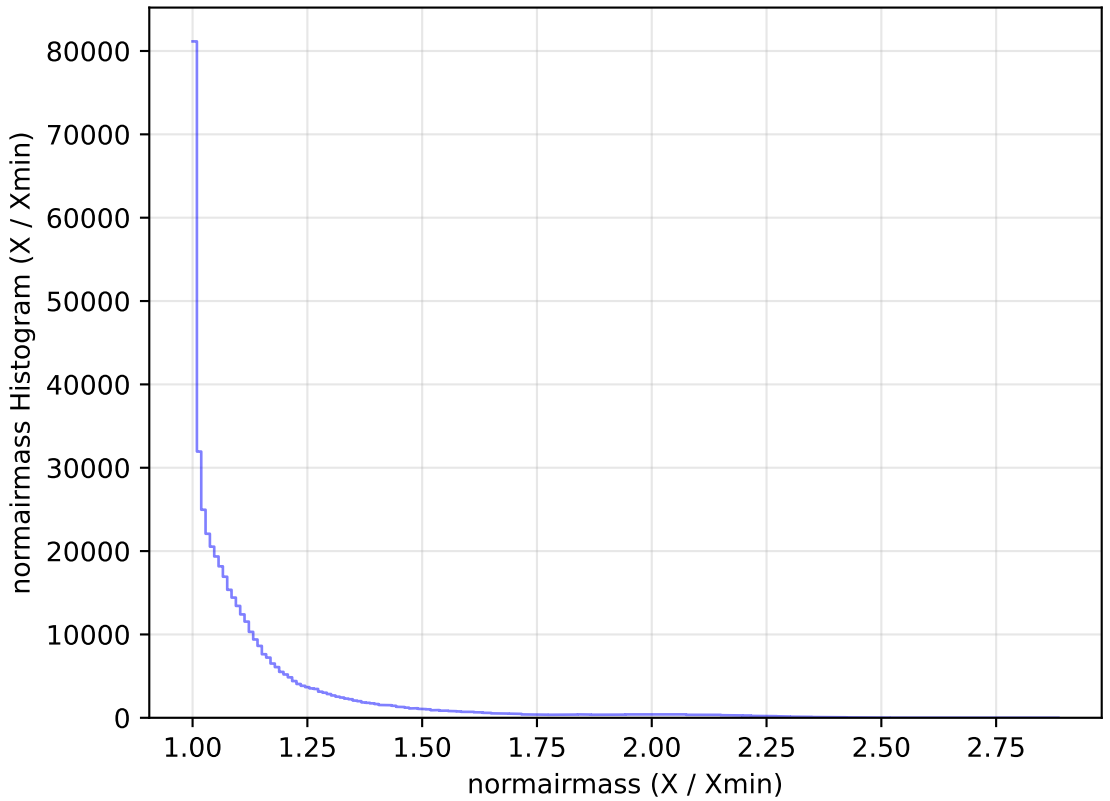
internal_u_expt27_nscale1.5v3.4_10yrs WFD r band: normairmass Histogram
