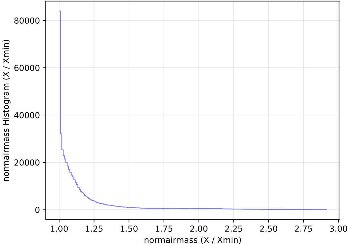
internal_u_expt27_nscale1.5v3.4_10yrs WFD i band: normairmass Histogram
