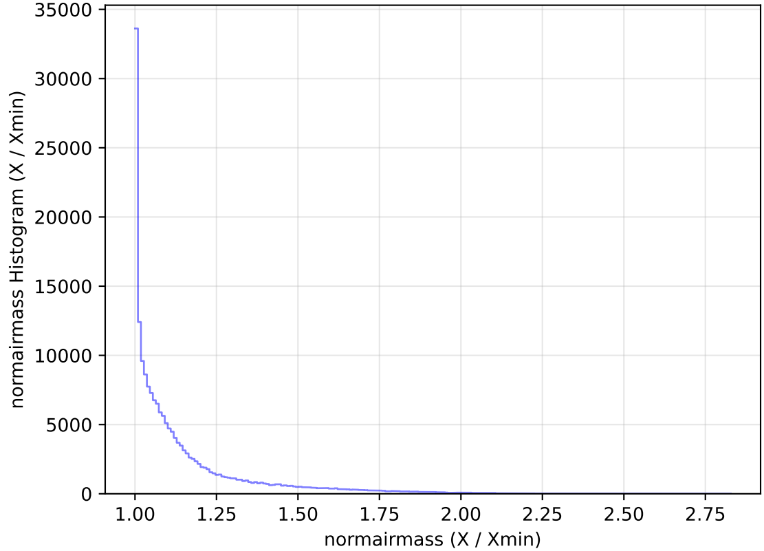
internal_u_expt27_nscale1.5v3.4_10yrs WFD g band: normairmass Histogram
